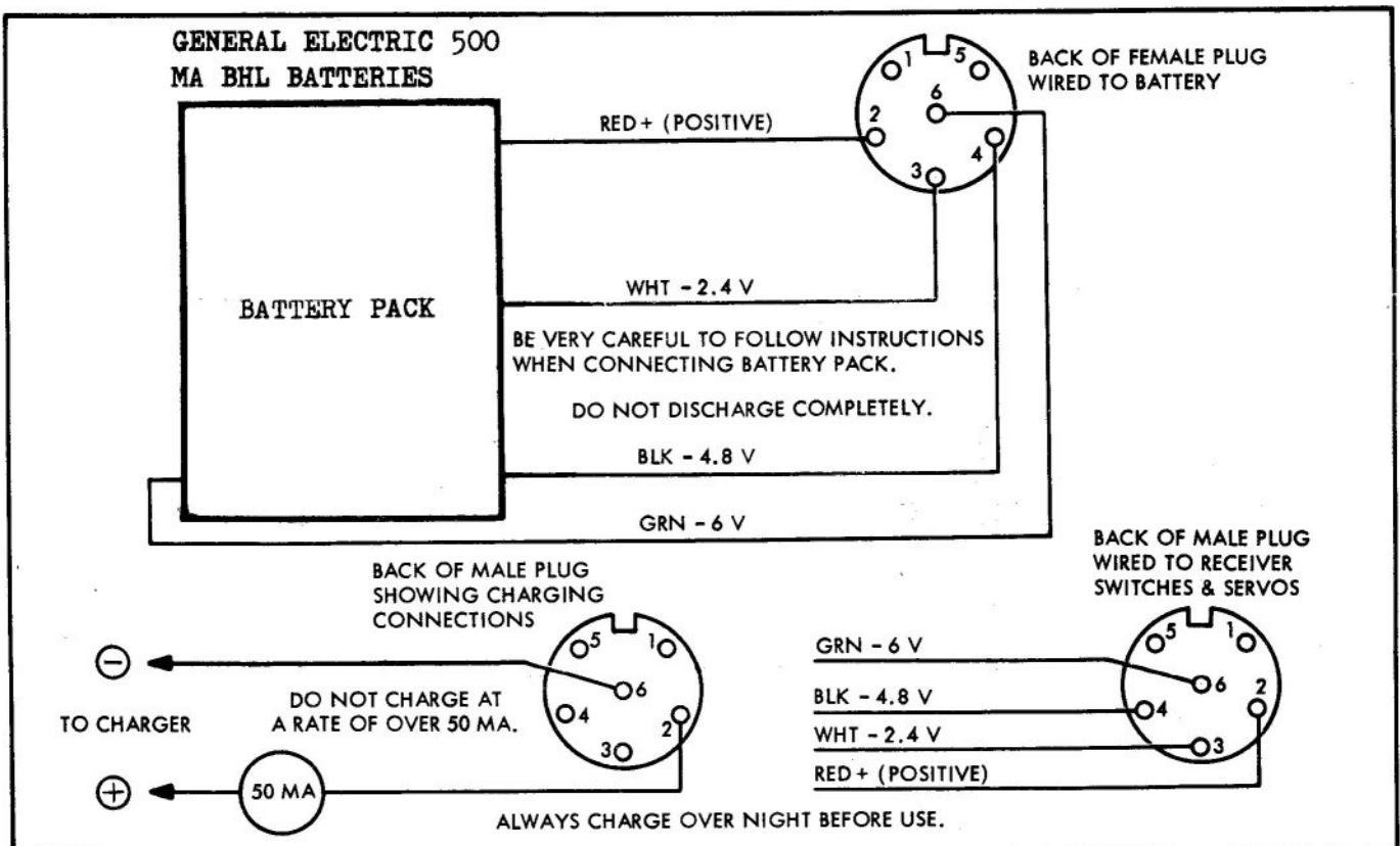
Wiring Diagram for KRAFT 6 Volt 500 MAH Battery Pack
