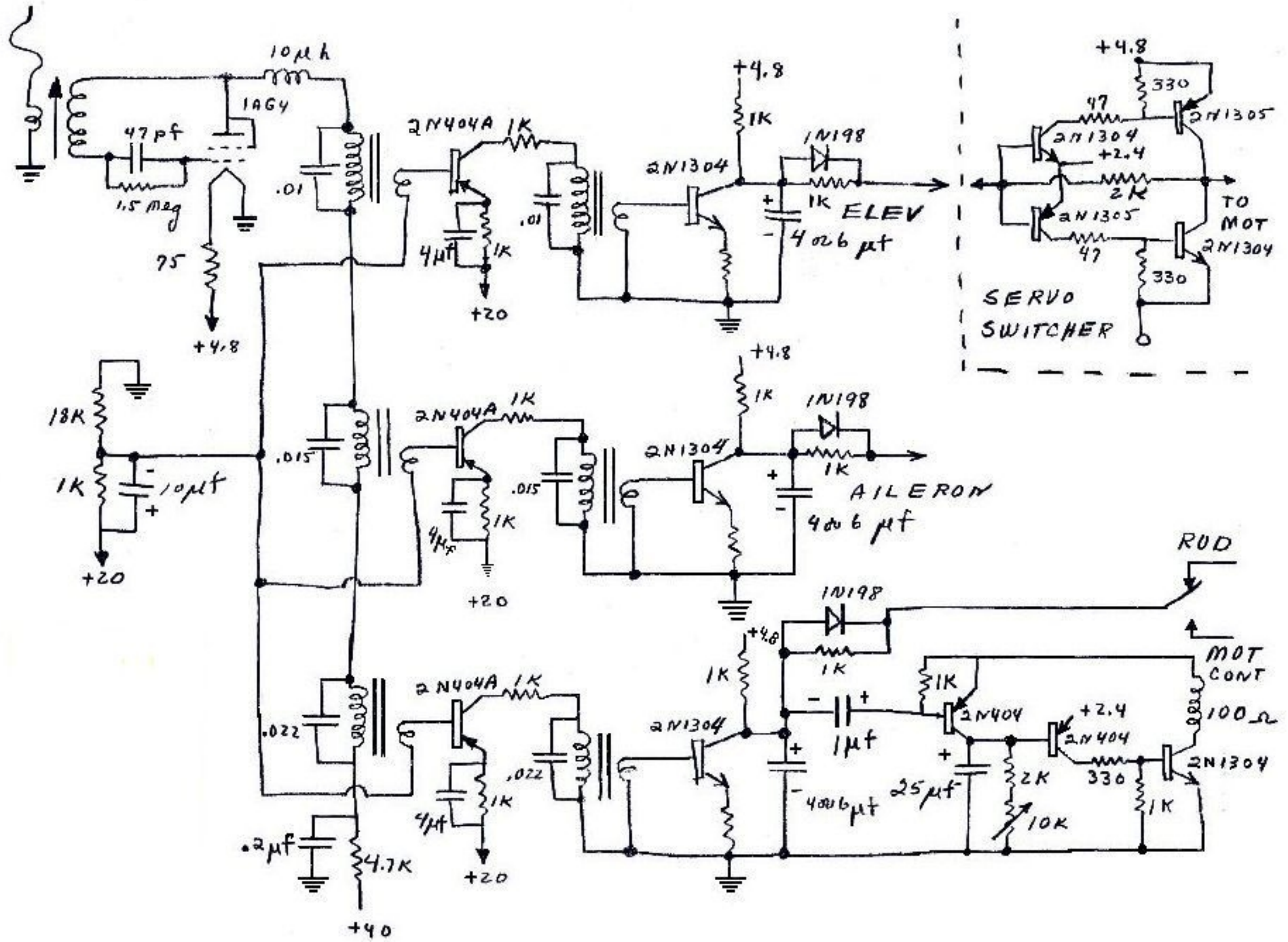
Quadruplex 21 superregen 50 MHz receiver
