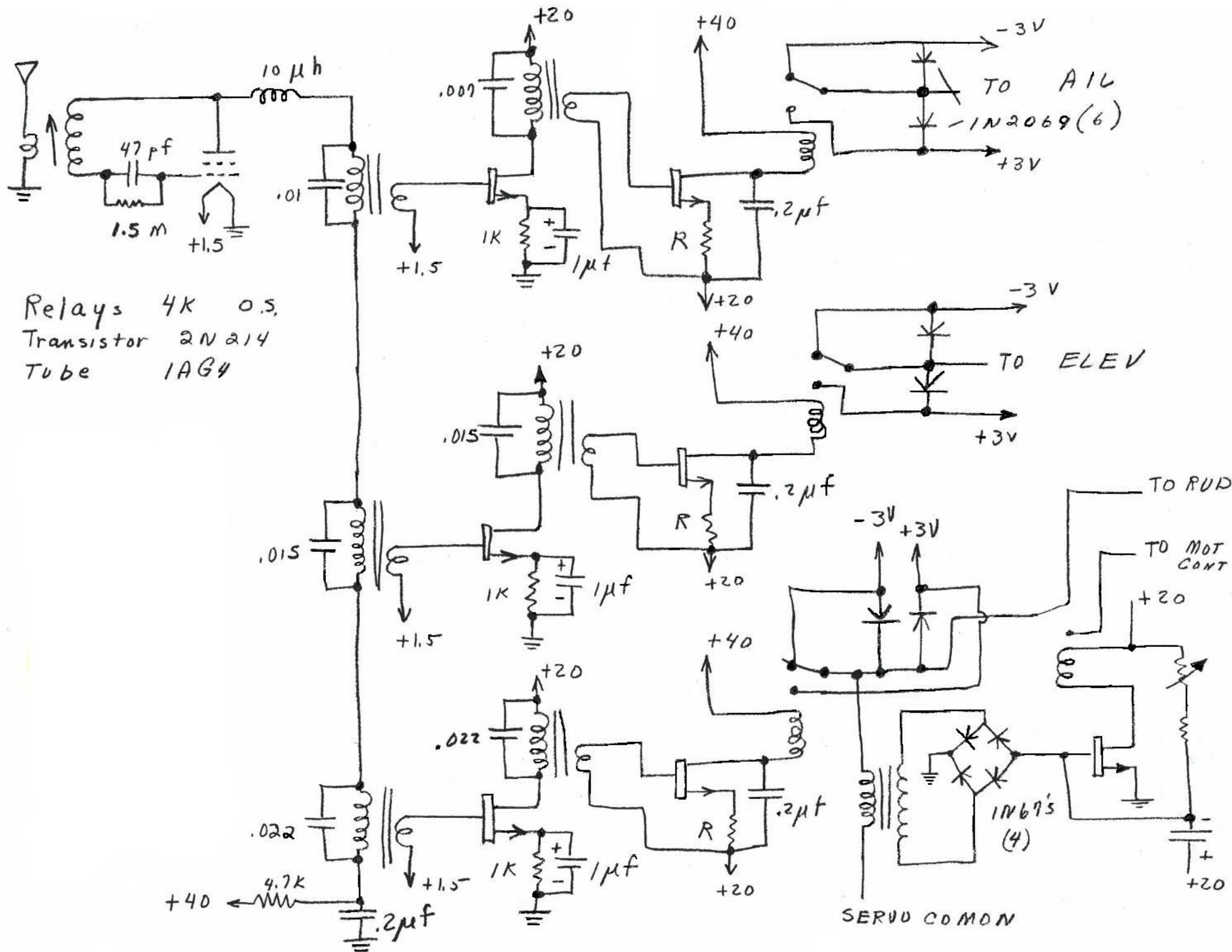
Quadruplex Mark I & II receiver
