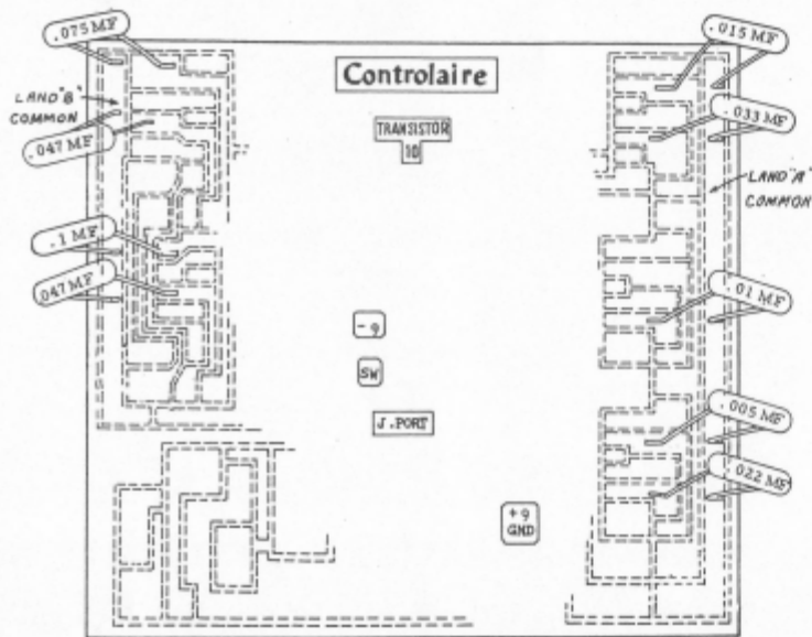
Fig. 1 TONE ALIGNMENT CONDENSER PLACEMENT
