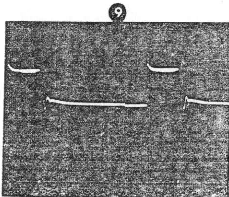
AMPLITUDE 4.5V (ERROR SIGNAL, STALLED CCW)
